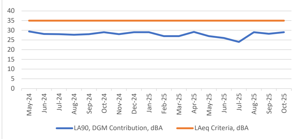
Figure 2 - Historic Noise Compliance Average - Dargues Gold Mine
