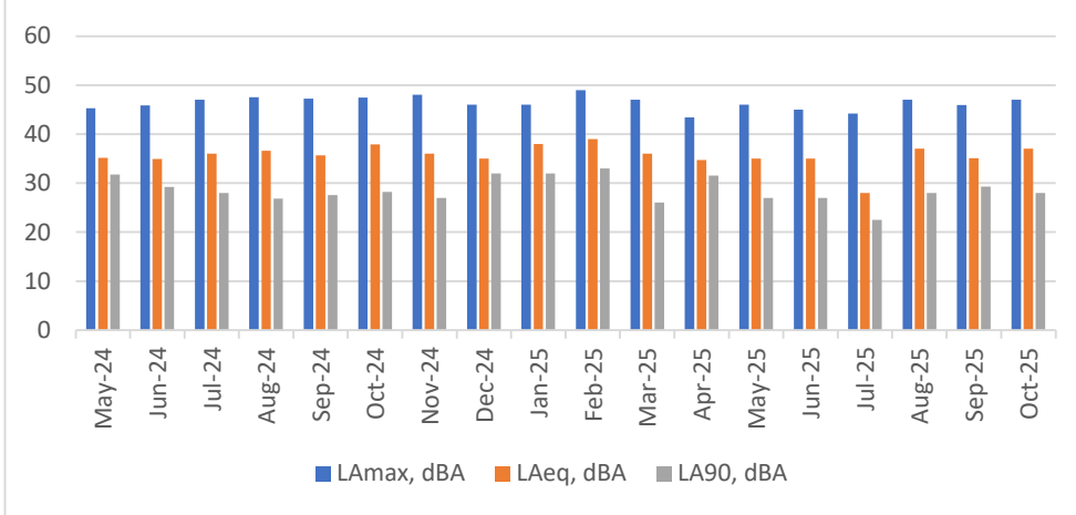
Figure 1 - Average Monthly Noise Metrics - Dargues Gold Mine
