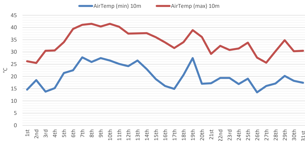
AIR TEMPERATURE DECEMBER 2023
