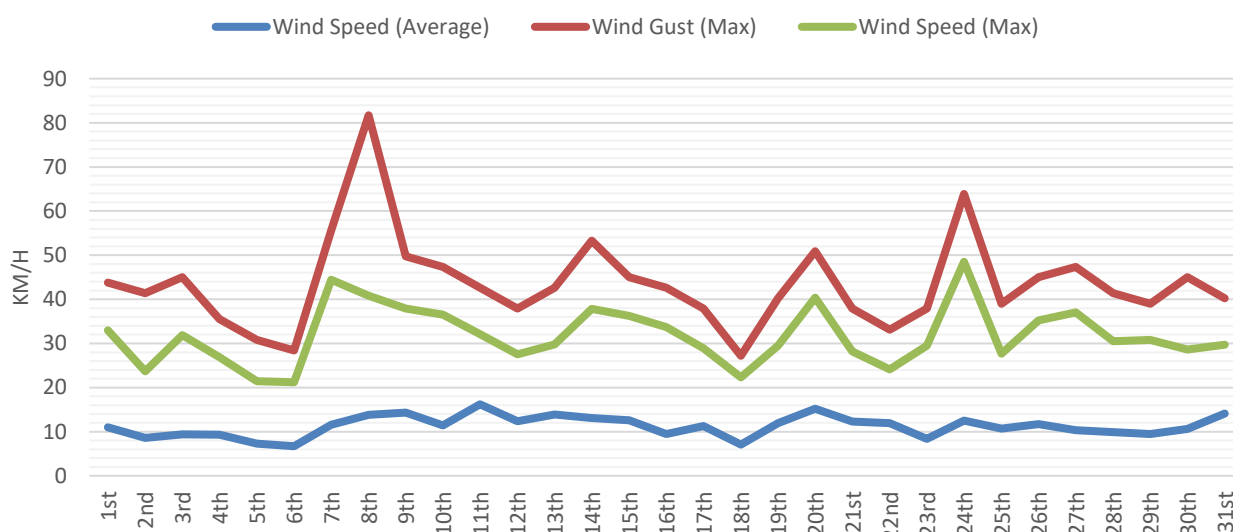
WIND SPEED DECEMBER 2023
