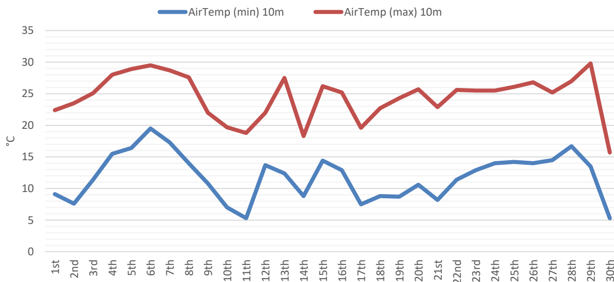
AIR TEMPERATURE APRIL 2023
