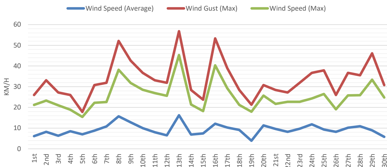
WIND SPEED APRIL 2023
