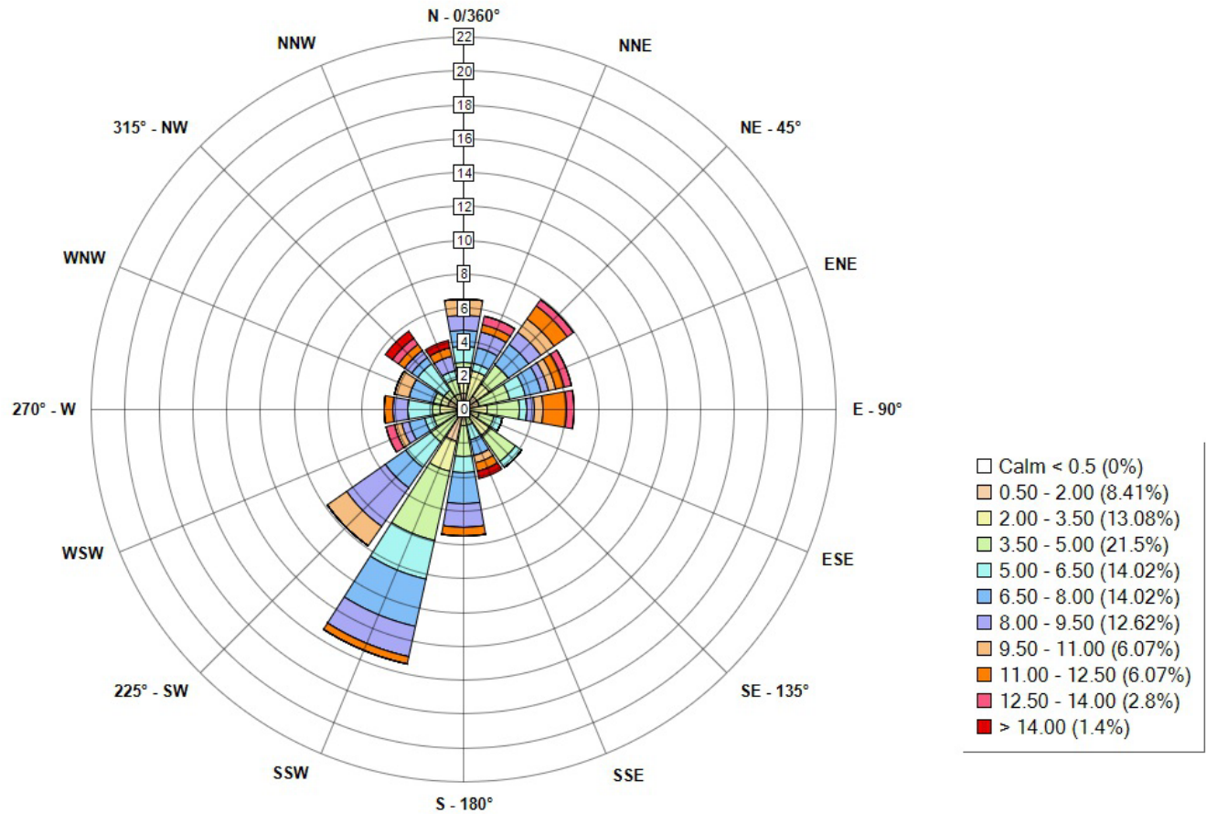
Wind Rose Report for: Hera Resources - Daily Summary VWDIR Inst. Wind Direction and VWSP Inst. Wind Speed in km/h Period: 2022-06-01 00:00 to 2022-12-31 23:59 Direction the Wind is Coming From
