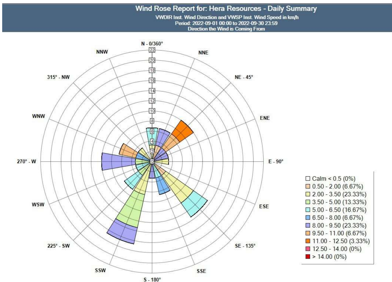
Figure 3 - Wind Rose for September 2022
