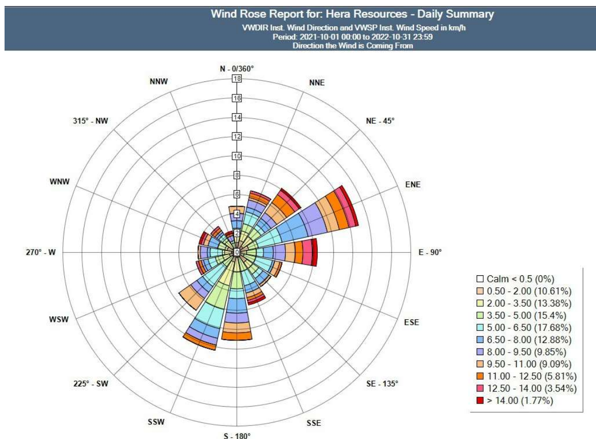
Figure 3 - Wind Rose for October 2022
