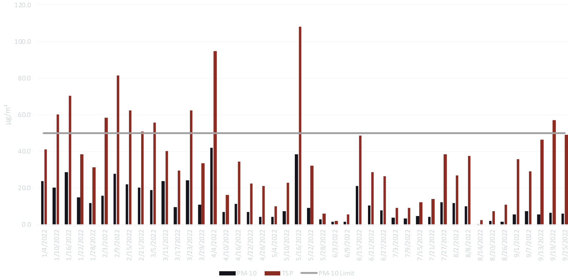
January 22 to September 22 - High Volume Air Sampler
