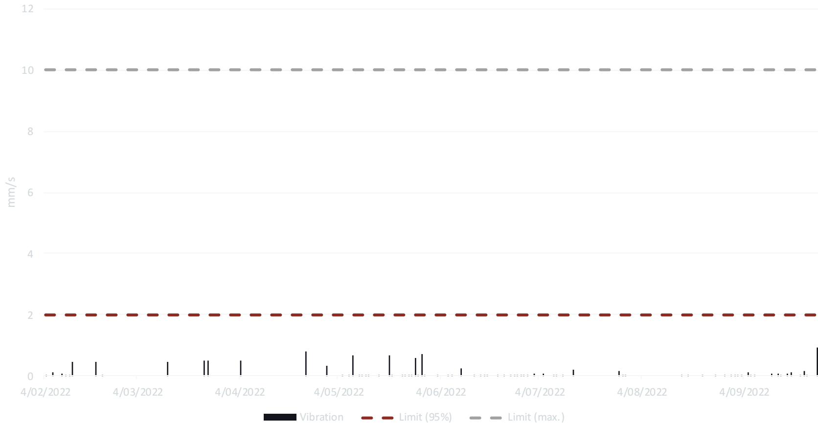
January 22 to September 22 - Blast Vibration (Evening Time Period)
