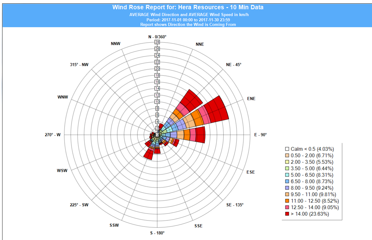
Figure 2. Wind rose November 2017.
