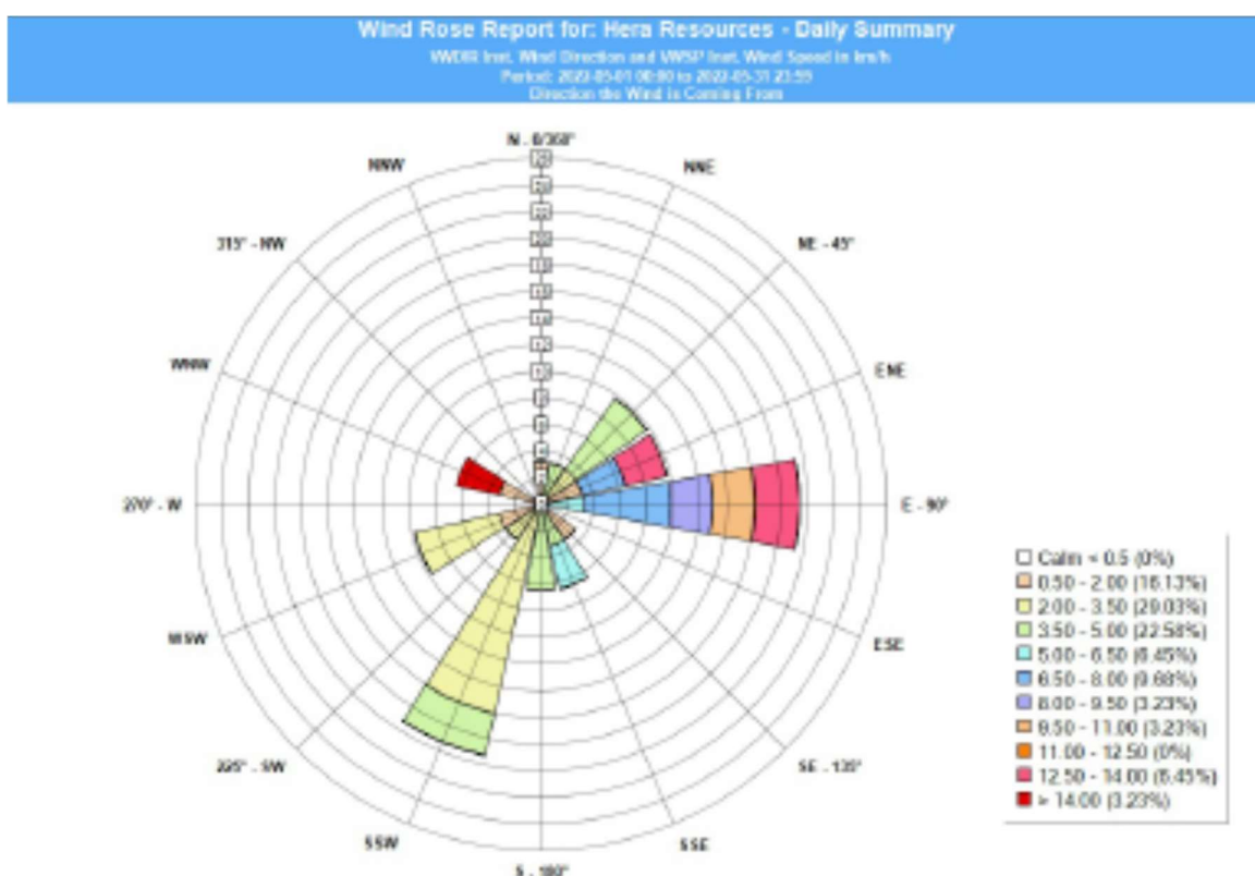
Figure 3 - Wind Rose for May 2022
