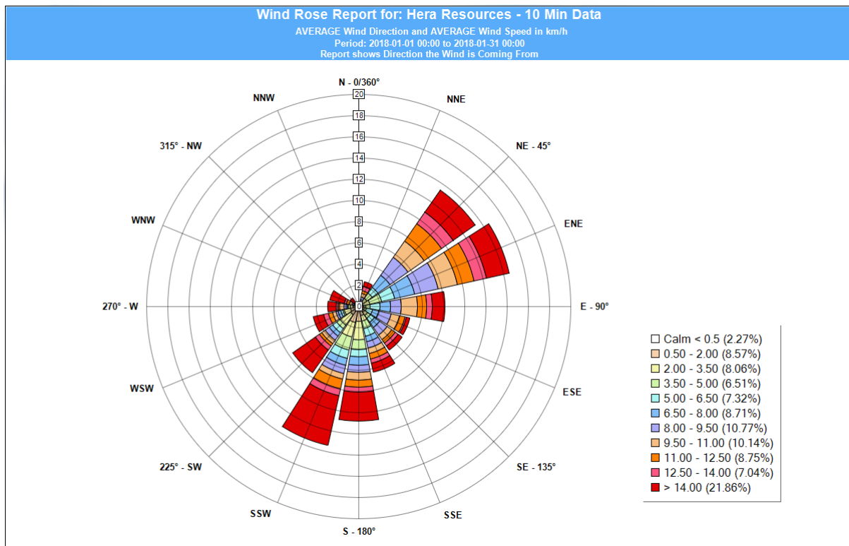
Figure 2. Wind rose January 2018.
