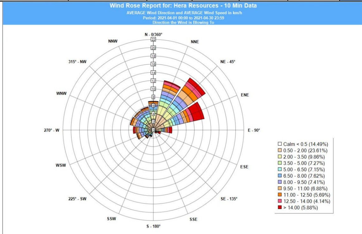
Figure 3 –Wind Rose Hera April 2021
