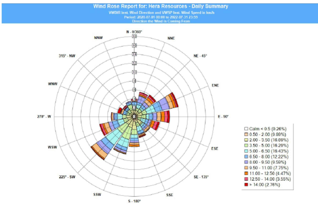
Figure 3 - Wind Rose for July 2022
