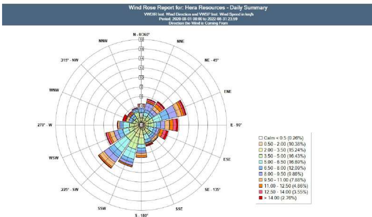
Figure 3 - Wind Rose for August 2022
